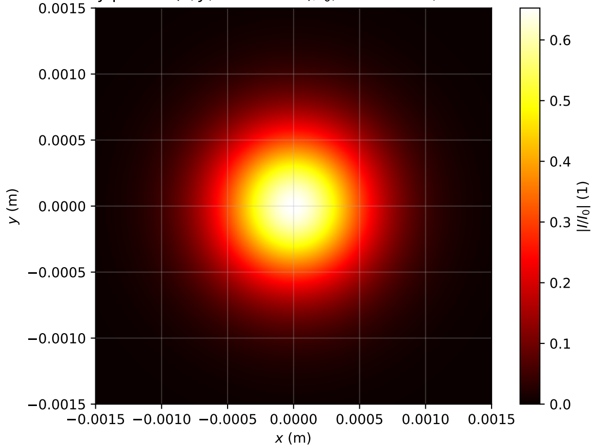
Intensity profile I(x, y, z = 2.627m)/I_0 , Pin=0.5Pcr, artificial time
